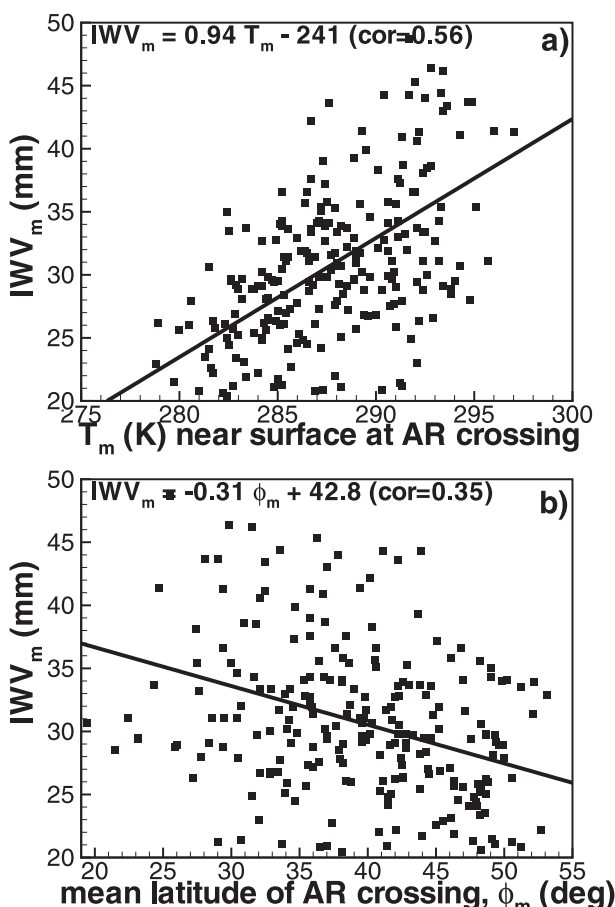
FIG. 5. The scatterplots between IWV_m and (a) the mean AR temperature near the surface T_m and (b) a mean latitude of an AR crossing \phi_m for the entire 2006–09 dataset.
